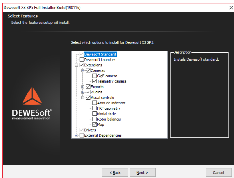
Figure 1: Feature selection
